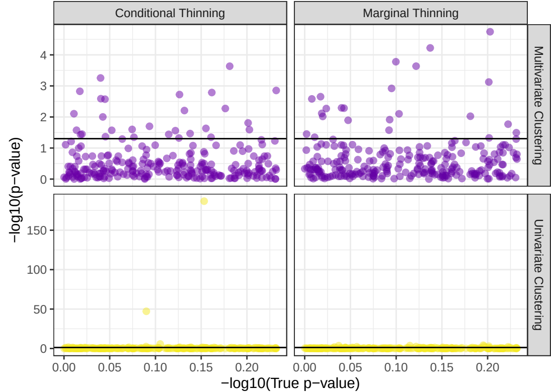
Distribution of p-values for genes under H_1
